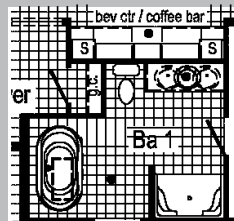
Optional Freestanding Tub & Shower
