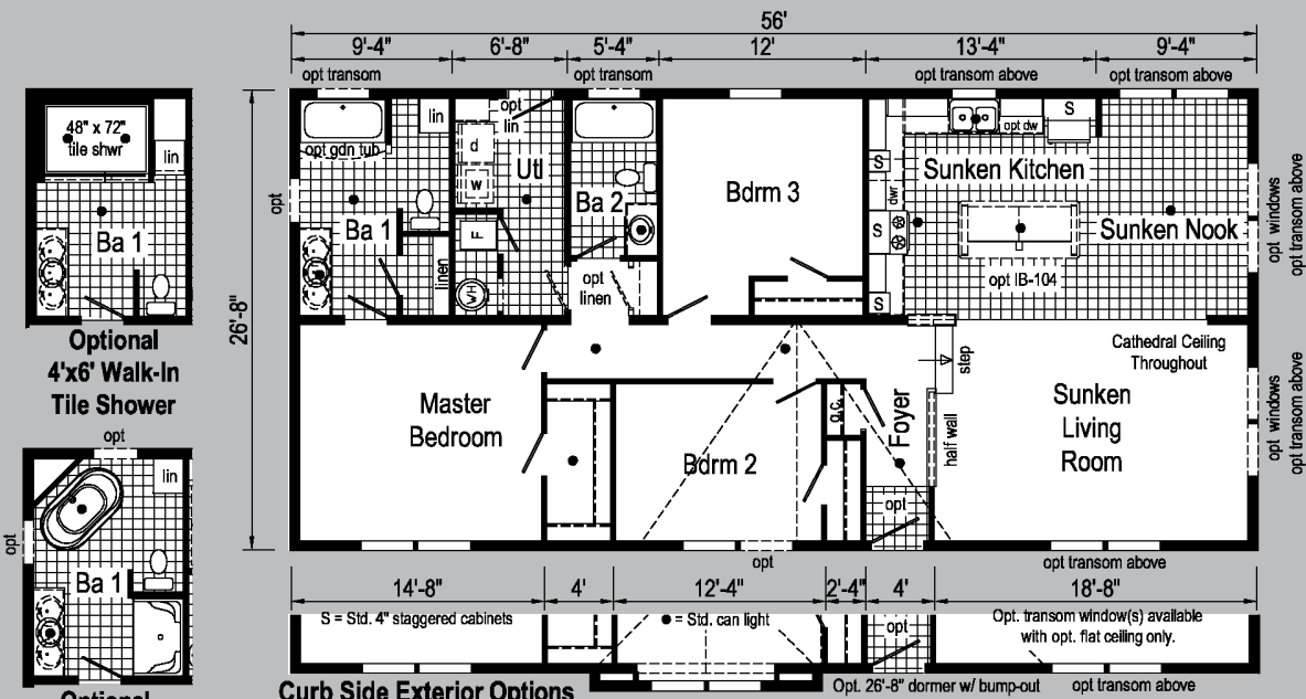
Optional Freestanding Tub with Shower (omits linen closet)
